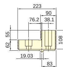
硬爪 HJ-50 for V-40"~79" Hardened jaw
